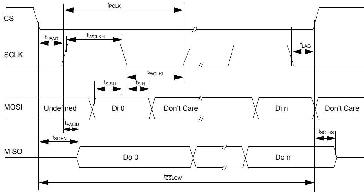
Figure 10. SPI Timings
