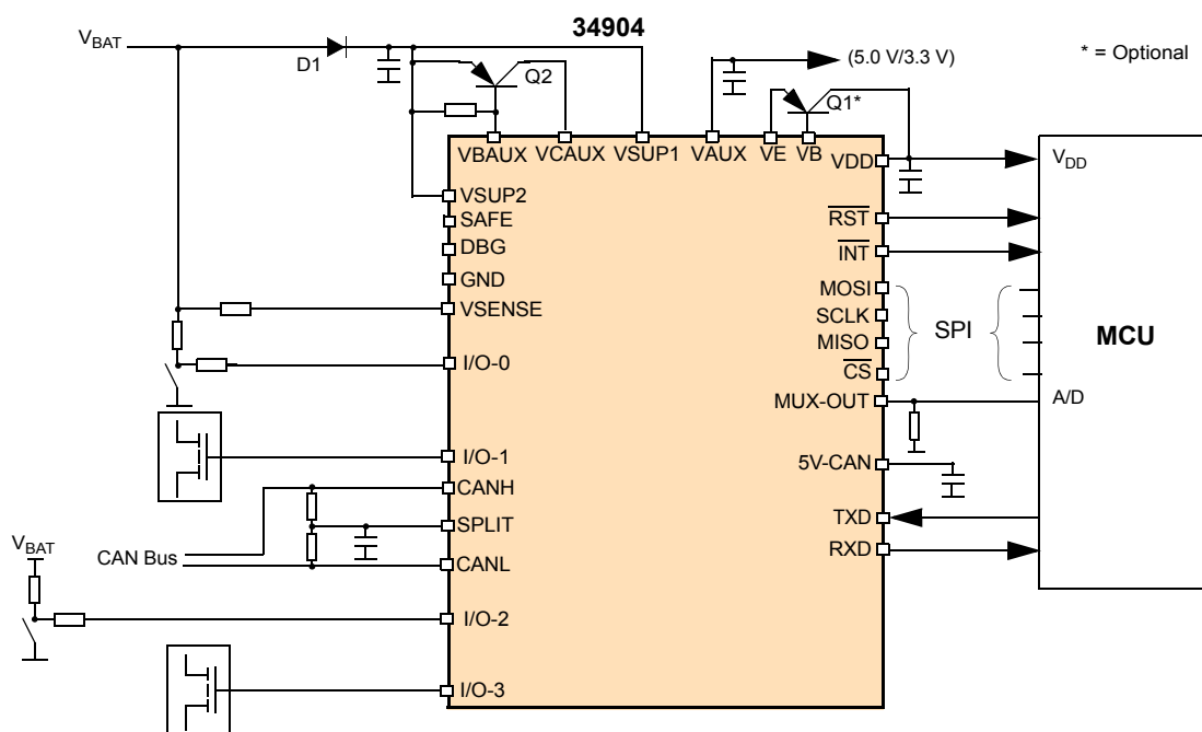
Figure 2. 34904 Simplified Application Diagram
